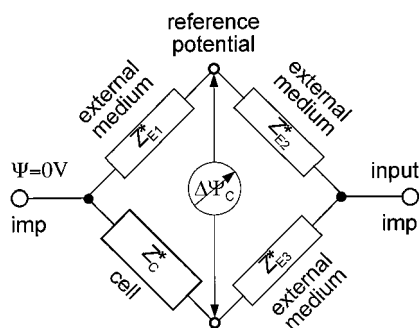
FIGURE 7 Redrawing of the RC model in Fig. 2. The figure demonstrates the Wheatstone bridge-like principle of the single cell methods DP and ER. Z_{e1} , Z_{e2} , and Z_{e3} stand for the IMPs of the three RC pairs e1, e2, e3, respectively, which describe the external solution. Z_c stands for the IMP of the cell (RC pairs i and m; see Fig. 2).
